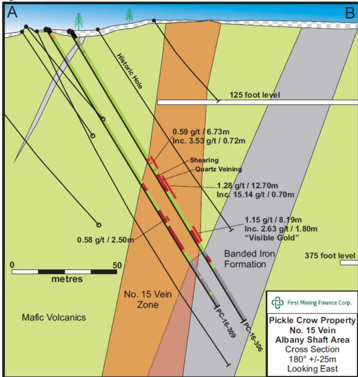
Figure 2. Cross-Section of No. 15 Vein
